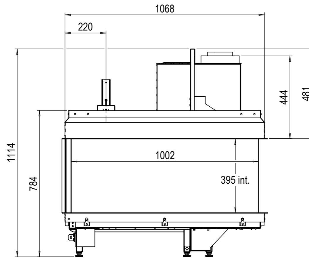
Dimensional drawing Respect Premium OC
