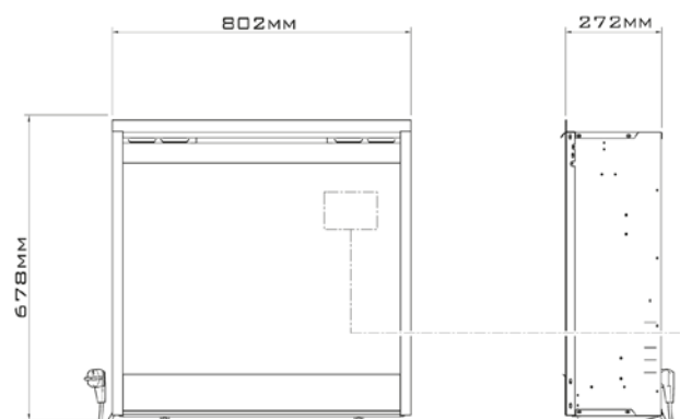
DF3020 – 30" firebox
